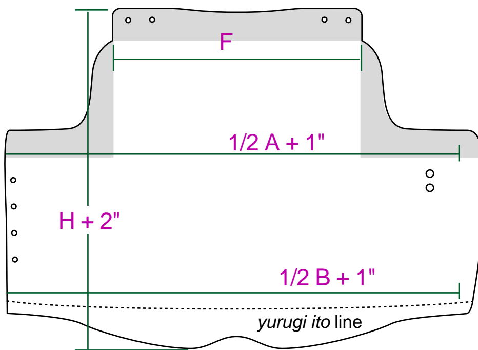
Back plate
