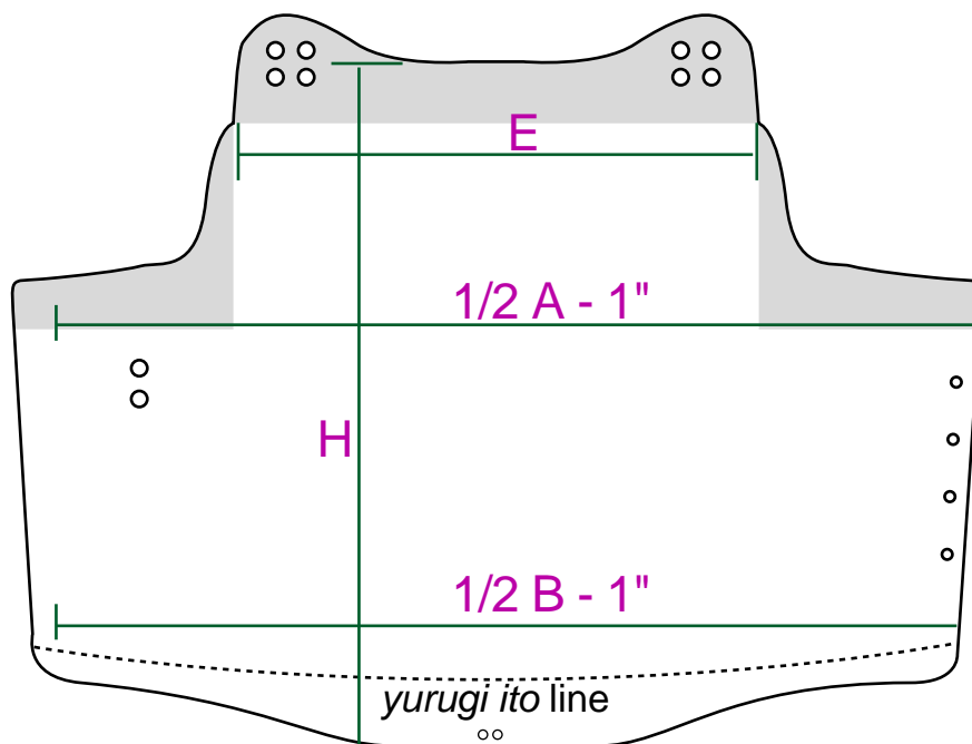
Front plate
